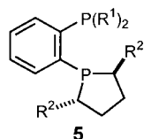
Figure 2. Possible coordination modes in intermediate [(3)][\text{Rh}(\text{P-P})]^+ complex and the dominant factor of enantioselectivity in the diposphine with 1,2-phenylene backbone.
