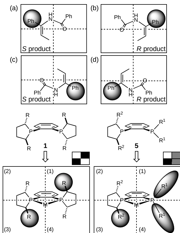
Figure 2. Possible coordination modes in intermediate [(3)][\text{Rh}(\text{P-P})]^+ complex and the dominant factor of enantioselectivity in the diposphine with 1,2-phenylene backbone.
