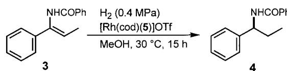
Scheme 1. Hydrogenation of ( Z )- N -benzoyl-1-phenylpropenamine 3 catalyzed by Rh complexes (see Table 1).
