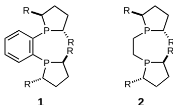
Figure 1. Structures of ligands 1 and 2 .
